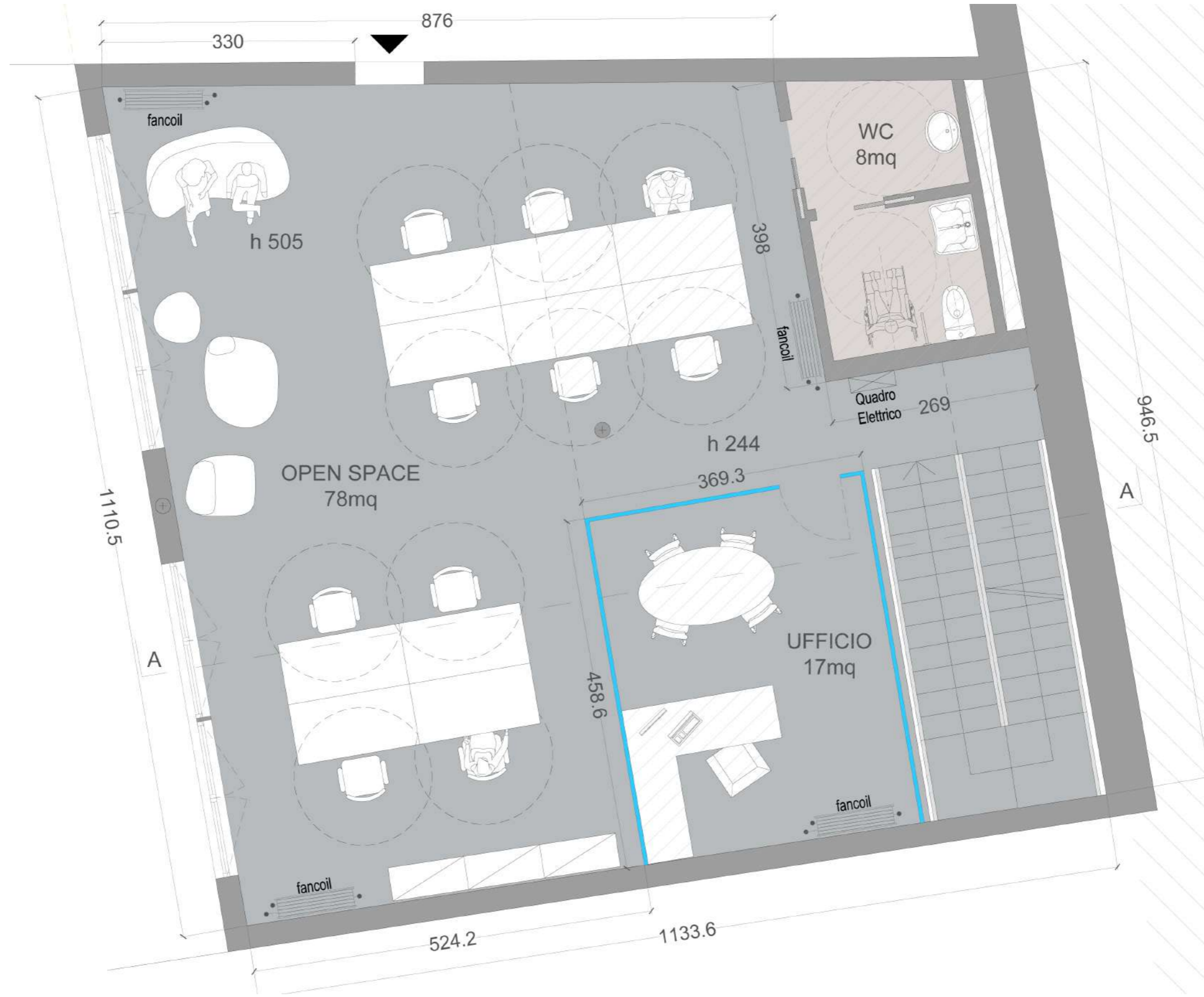
PIANTA – Piano Primo PLAN – First Floor
